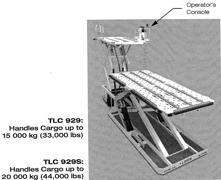
Figure 1: Dual-platform Scissor Lifts
