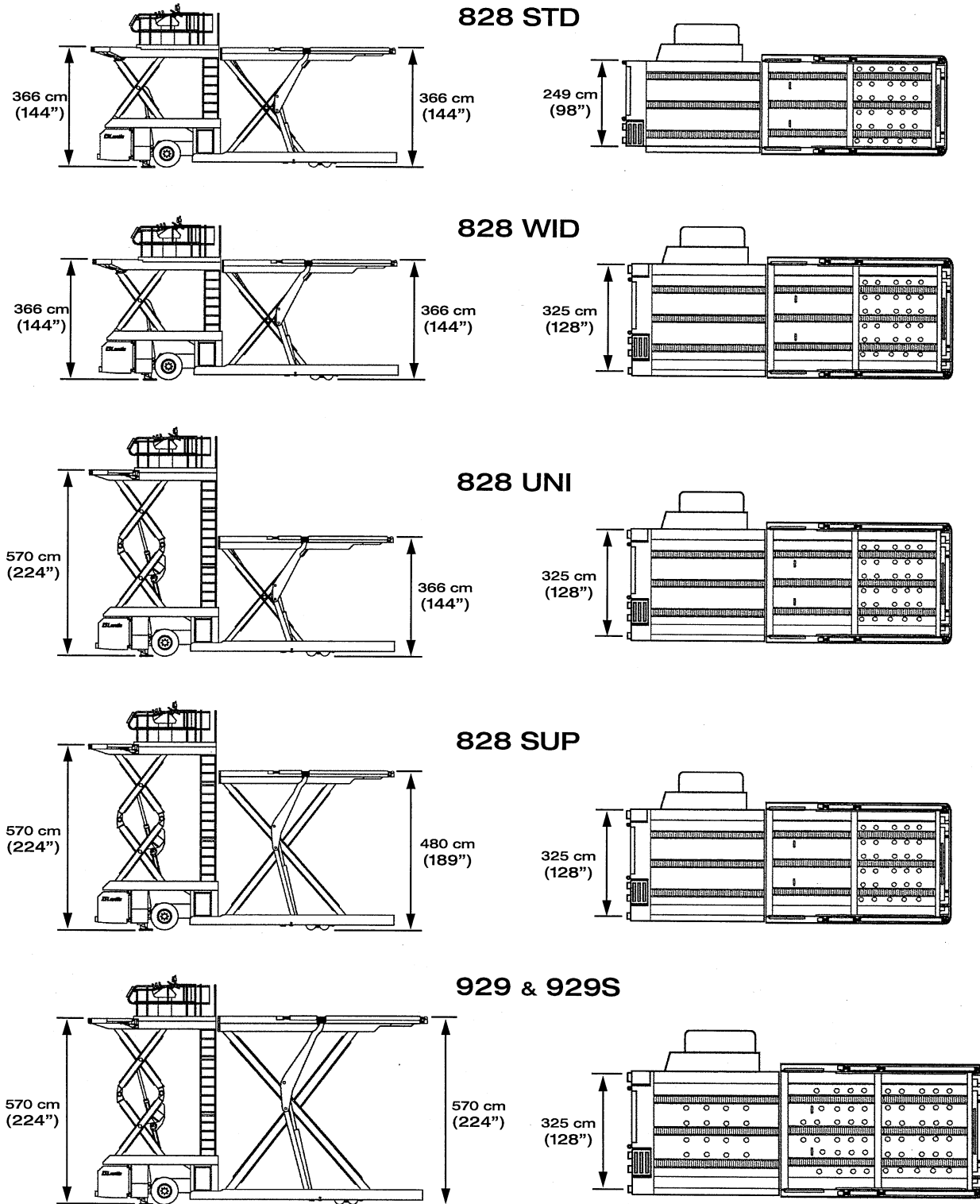
Figure 5: TLC 828 and TLC 929 Models
